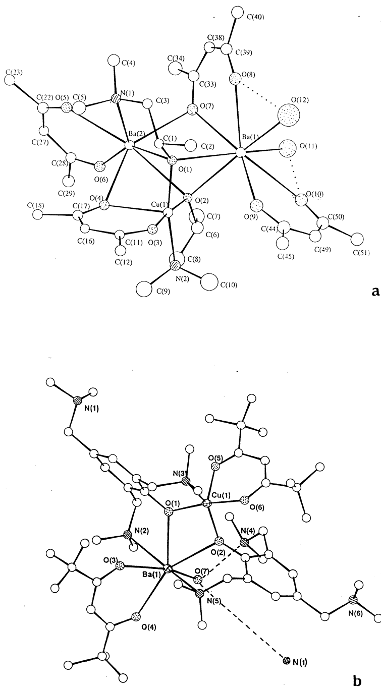
Fig. 8. (a) Molecular structures of Ba-Cu heteroleptic species: (a) [\text{Ba}_2\text{Cu}(\mu_3, \eta^2\text{-OR}_N)_2(\mu, \eta^2\text{-thd})_2(\eta^2\text{-thd})(\text{Pr}^i\text{OH})_2] ; (b) [\text{BaCu}(\text{thd})_2(\text{O-tamp})_2(\text{H}_2\text{O})] \text{Ba} \cdots \text{Cu} = 3.680(3) ; \text{Ba-O} = 2.57(2), 2.67(1), 2.11(2) ; \text{Cu-N} = 2.14(2) .
