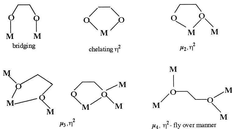
Scheme 3. Coordination modes of diolates, especially ethyleneglycolates.
