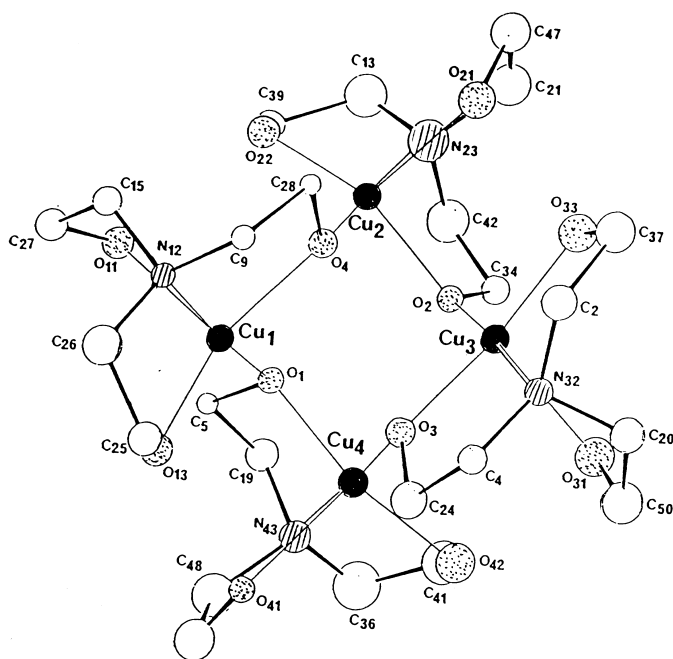
Fig. 6. Ball-and-stick drawing of the tetranuclear core of [\text{Cu}(\mu\text{-teaH}_2)]_4 \cdot 3\text{teaH}_3 [ \text{Cu}-\text{O}=1.85(3)\text{--}2.47(4) ] [ \text{Cu}(4)-\text{O}(41) ], \text{Cu}-\text{N}=1.89(6)\text{--}2.09(6) Å.
