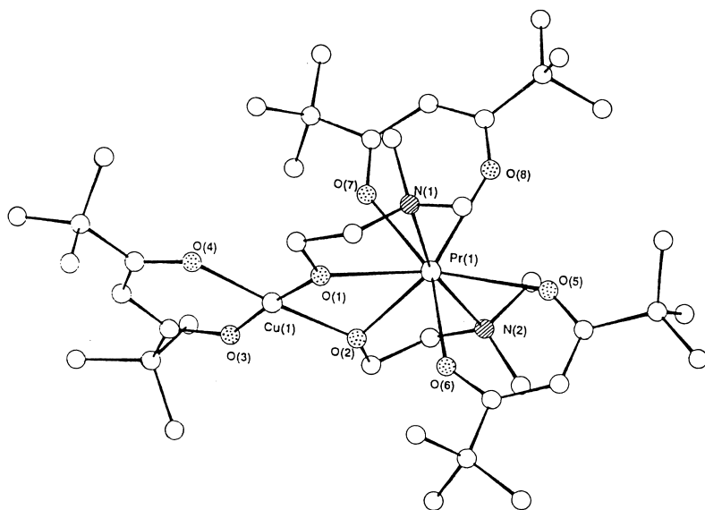
Fig. 10. Molecular structure of \text{PrCu}(\mu, \eta^2\text{-OCHMeCH}_2\text{NMe}_2)_2(\eta^2\text{-thd})_3 . Selected distances (Å): \text{Pr} \cdots \text{Cu} = 3.345(1) ; \text{Pr}-\text{N} = 2.695(9) av.; \text{Pr}-\text{O} = 2.368(7)\text{--}2.460(7) ; \text{Cu}-\text{O} = 1.896(7)\text{--}1.910(7) .
