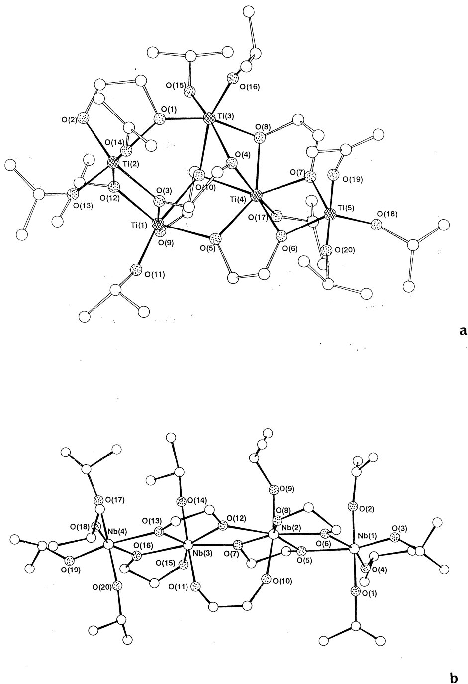
Fig. 4. (a) Molecular structure of \text{Ti}_5(\text{OPr}^i)_9(\mu\text{-OPr}^i)(\mu, \eta^2\text{-OC}_2\text{H}_4\text{O})(\mu_3, \eta^2\text{-OC}_2\text{H}_4\text{O})_3(\mu_4, \eta^2\text{-OC}_2\text{H}_4\text{O}) ; (b) Ball-and-stick drawing of the molecular structure of \text{Nb}_4(\mu, \eta^2\text{-OC}_2\text{H}_4\text{O})_4(\mu\text{-OC}_2\text{H}_4\text{O})(\text{OPr}^i)_{10} .
